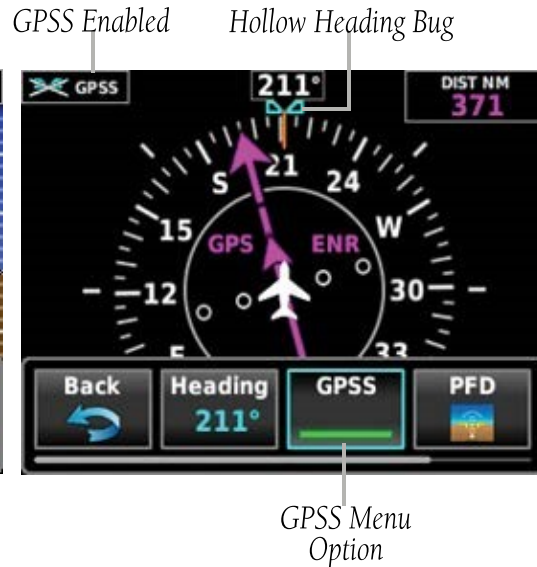
Figure 4-4 GPSS Enabled (HSI Page)
